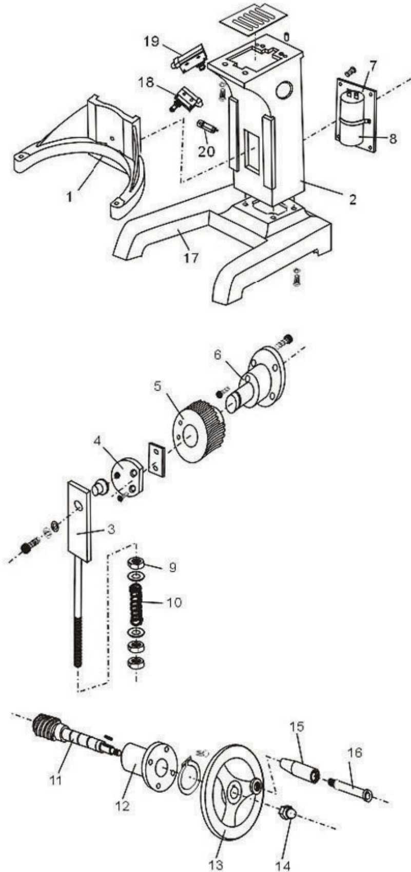
MACHINE SEAT, STAND & HANDWHEEL BOWL LIFTER UNIT - FIG 7
