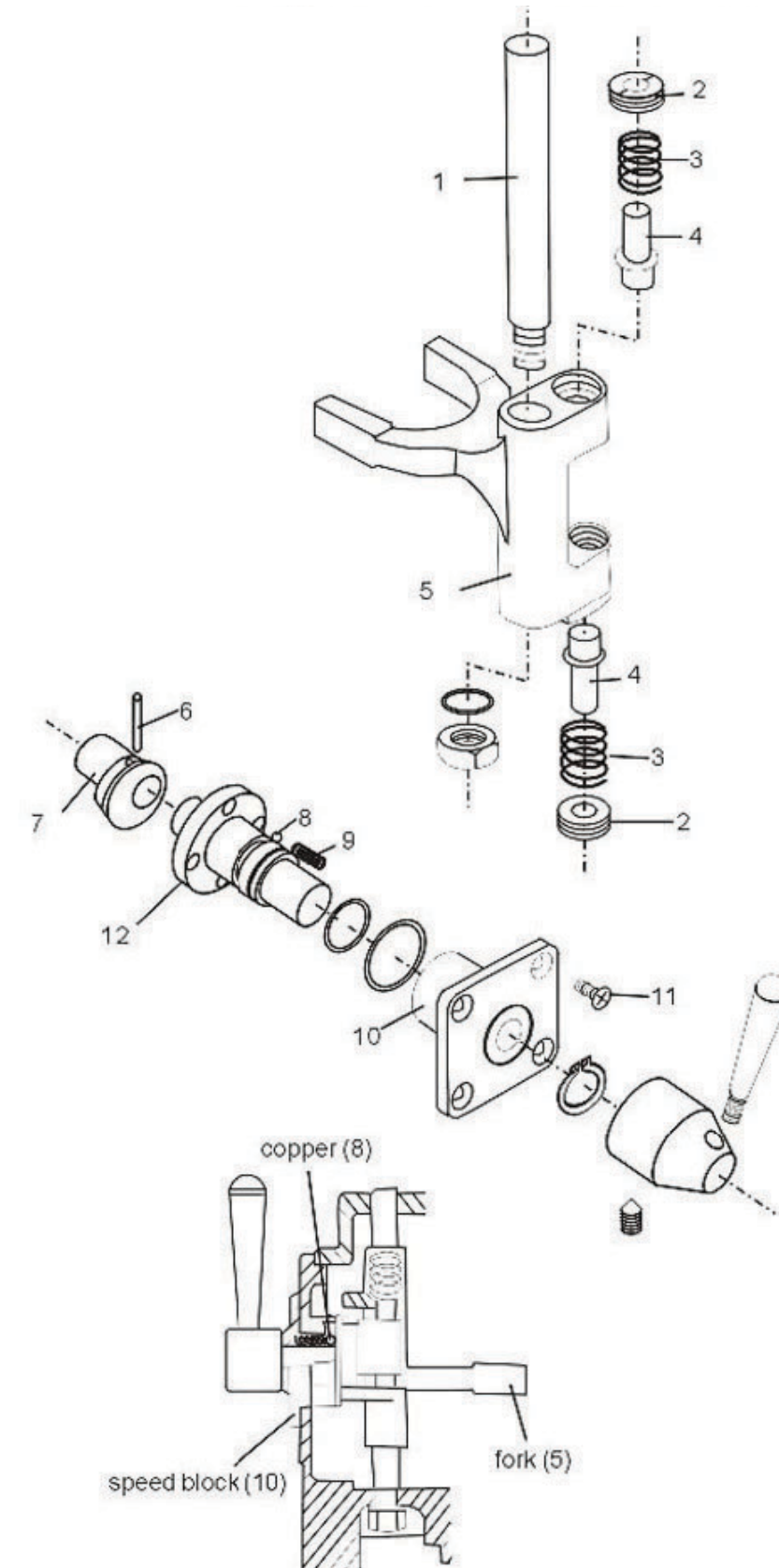
FORK & SPEED SHAFT - FIG 6
