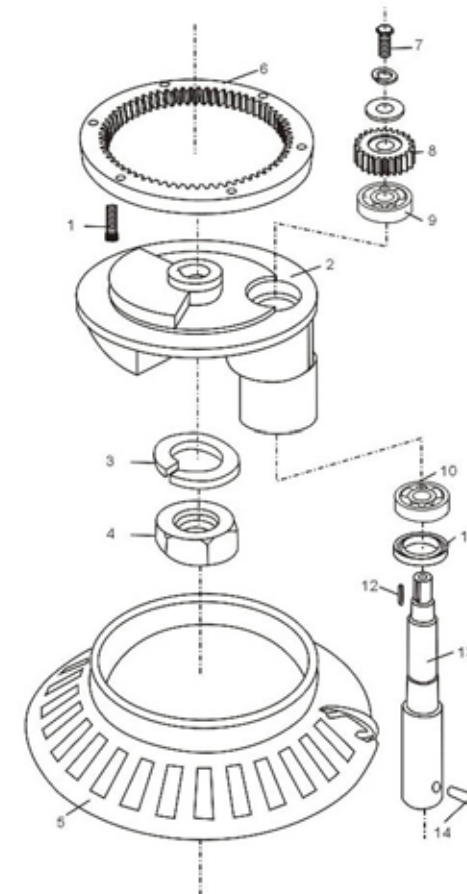
TURNING PLATE AND MIXING AXLE - FIG 9
