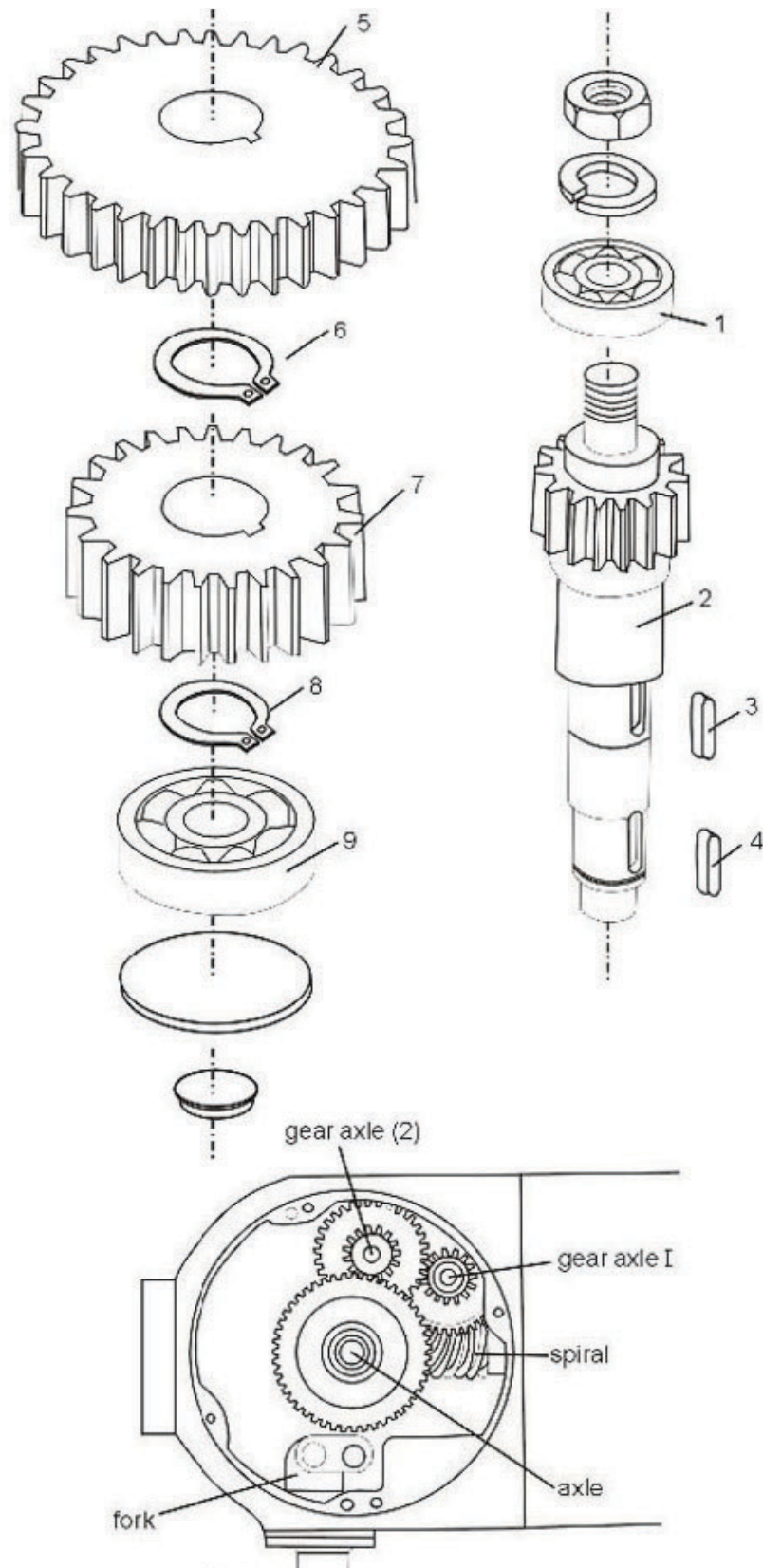
GEAR AXLE - FIG 3
