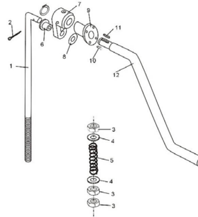
TURNING PLATE AND MIXING AXLE - FIG 9
